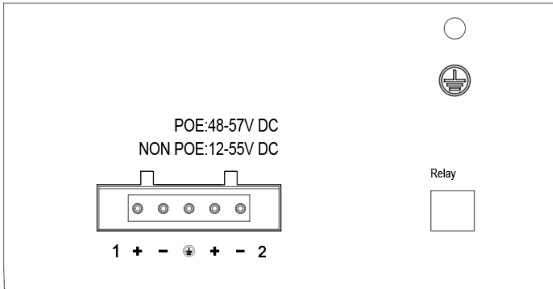
Figure 3-2 8-Port Gigabit+2G SFP Switch side panel
