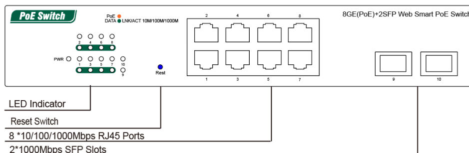
Figure 2-1 Front panel of the 8GE (PoE)+2SFP Switch
