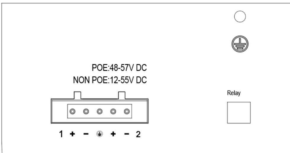
Figure 3-2 8-Port Gigabit+4GE Switch side panel
