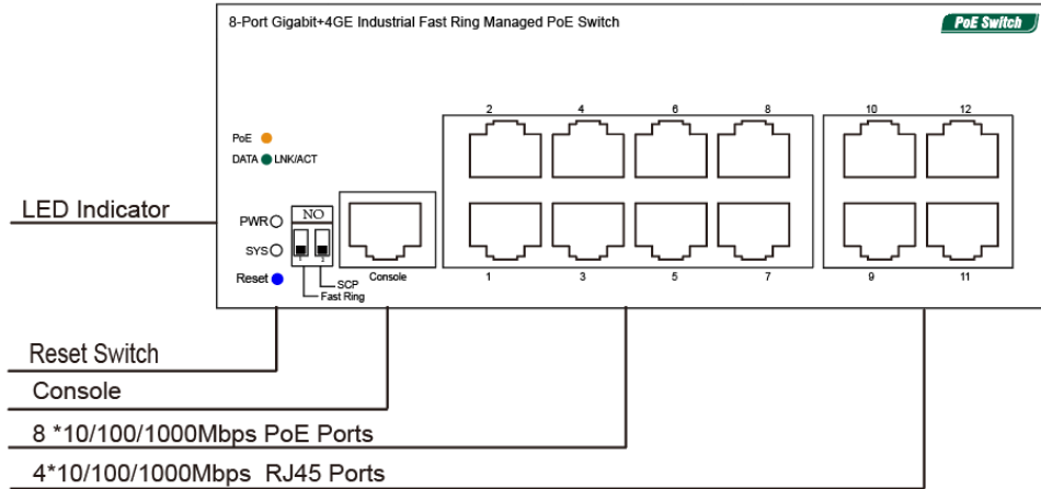
Figure 3-1 Front panel of the 8-Port Gigabit+4GE Switch
