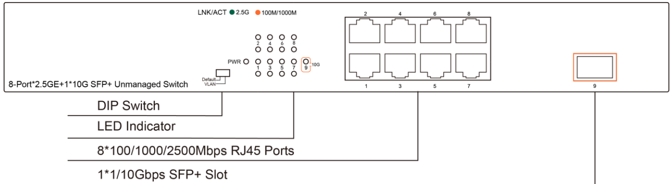
Figure 2-1 Switch front panel diagram
