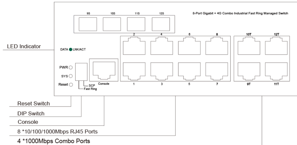
Figure 3-1 Front panel of the 8-Port Gigabit + 4G Combo Switch
