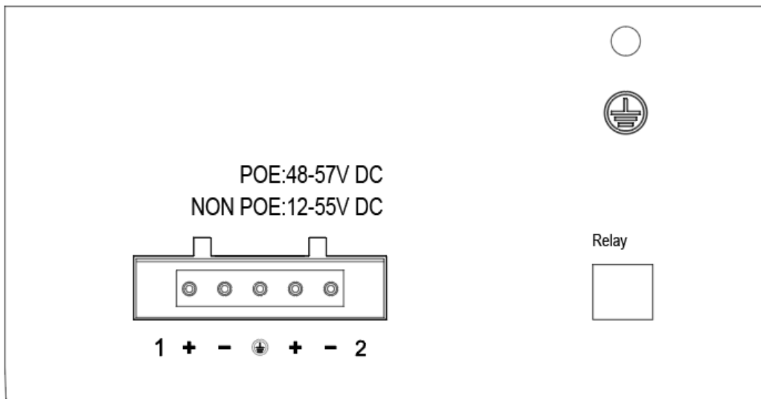
Figure 3-2 8-Port Gigabit + 4G Combo Switch side panel
