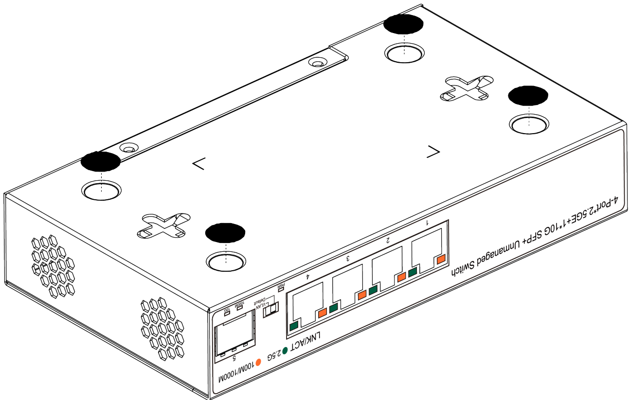
Figure 3-1 Desktop Installation Diagram
