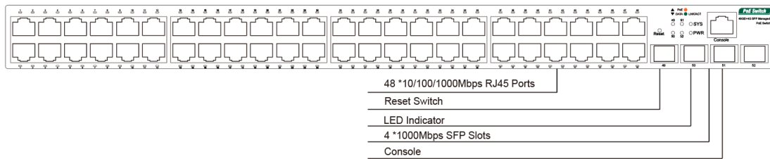
Figure 2-1 Front panel of the 48GE (PoE)+4G SFP Switch
