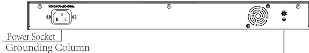
Figure 2-2 Rear panel of the 48GE (PoE)+4G SFP Switch
