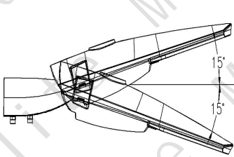
Luminaire tilt adjustment side entry:-15°to+15°
