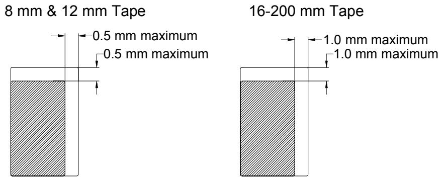
Figure 10 -- Bar code label area for punched and embossed carrier
