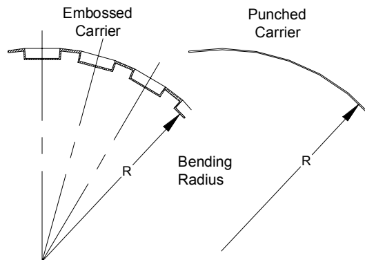
Figure 11 -- Bending radius for punched and embossed carrier
