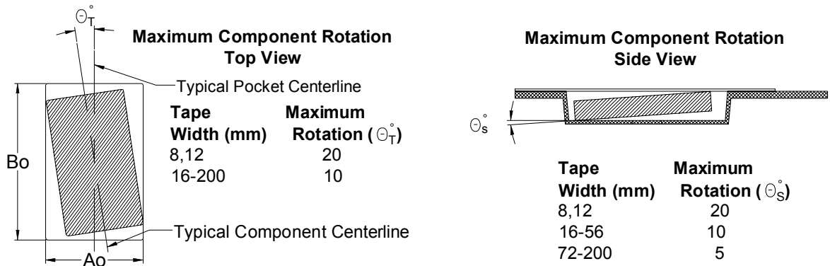
Figure 9 -- Maximum lateral movement for punched and embossed carrier
