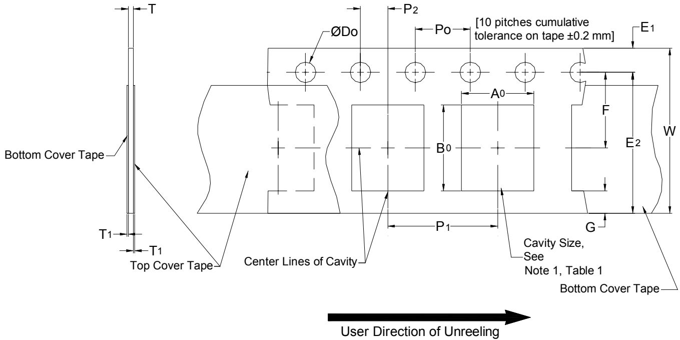
Figure 5 -- Illustration of 2 mm cavity pitch for 8 mm & 12 mm punched and embossed carrier, P1. See Tables 1 & 2 and requirement 4.3
