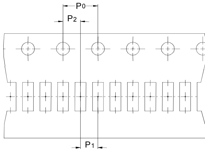
Figure 5 -- Illustration of 2 mm cavity pitch for 8 mm & 12 mm punched and embossed carrier, P1. See Tables 1 & 2 and requirement 4.3
