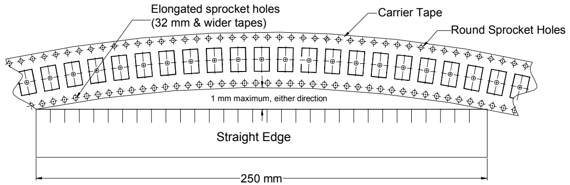
Figure 12 -- Maximum camber for punched and embossed carrier
